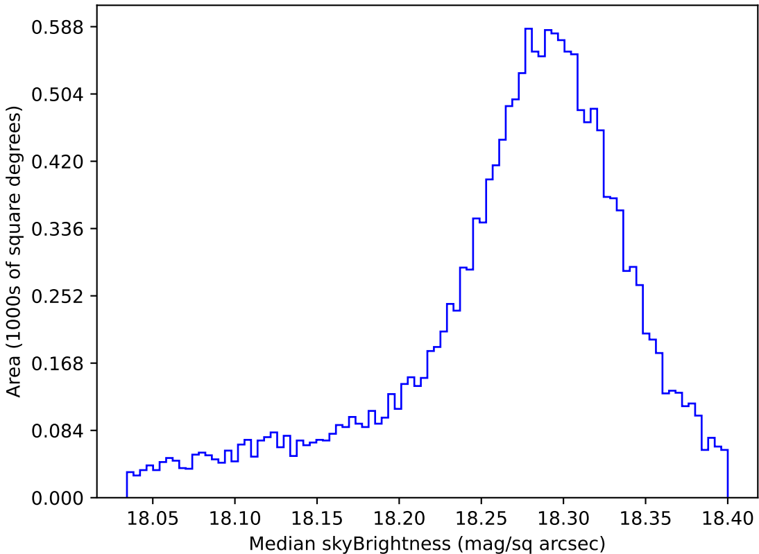
roll_pause_mjdp60_v3.4_10yrs WFD y band: Median skyBrightness
