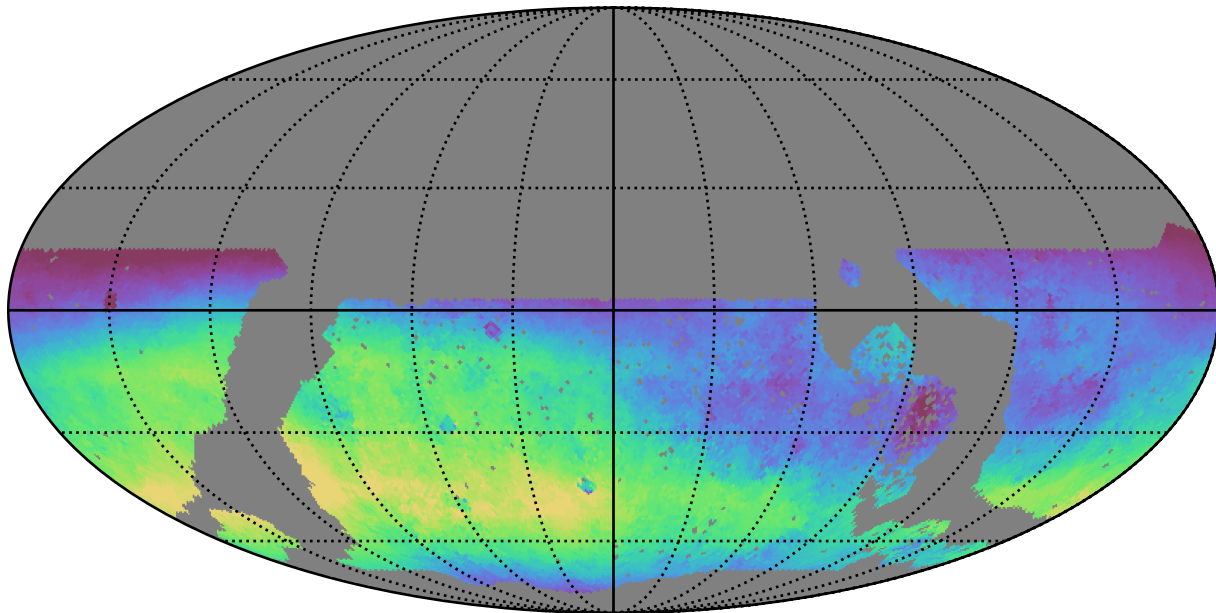
roll_pause_mjdp60_v3.4_10yrs WFD u band: Median skyBrightness
