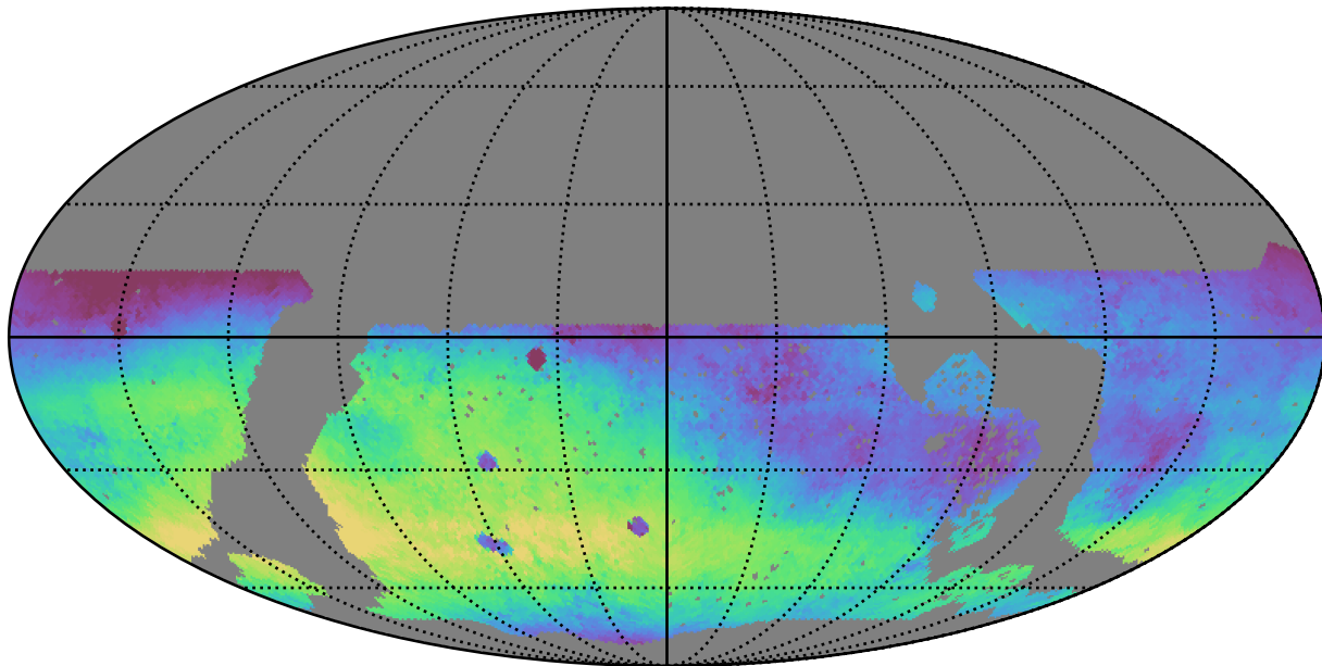
roll_pause_mjdp60_v3.4_10yrs WFD r band: Median skyBrightness
