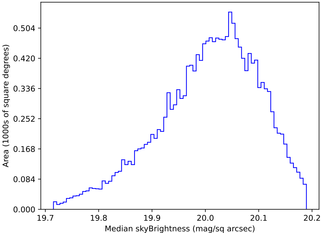
roll_pause_mjdp60_v3.4_10yrs WFD i band: Median skyBrightness
