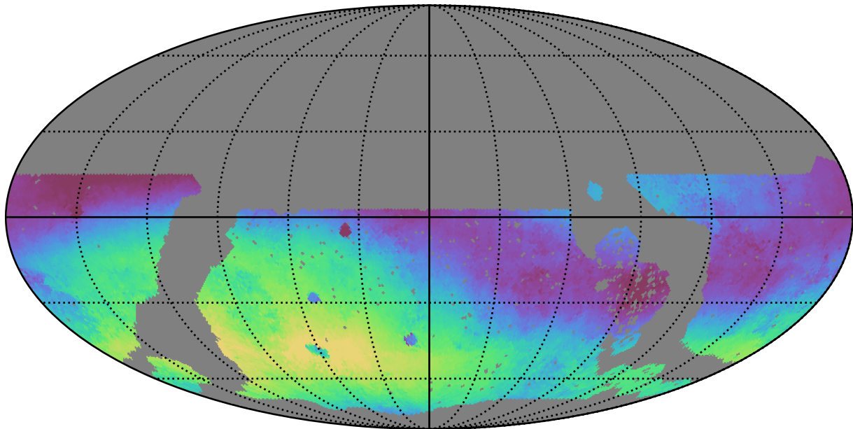
roll_pause_mjdp60_v3.4_10yrs WFD g band: Median skyBrightness
