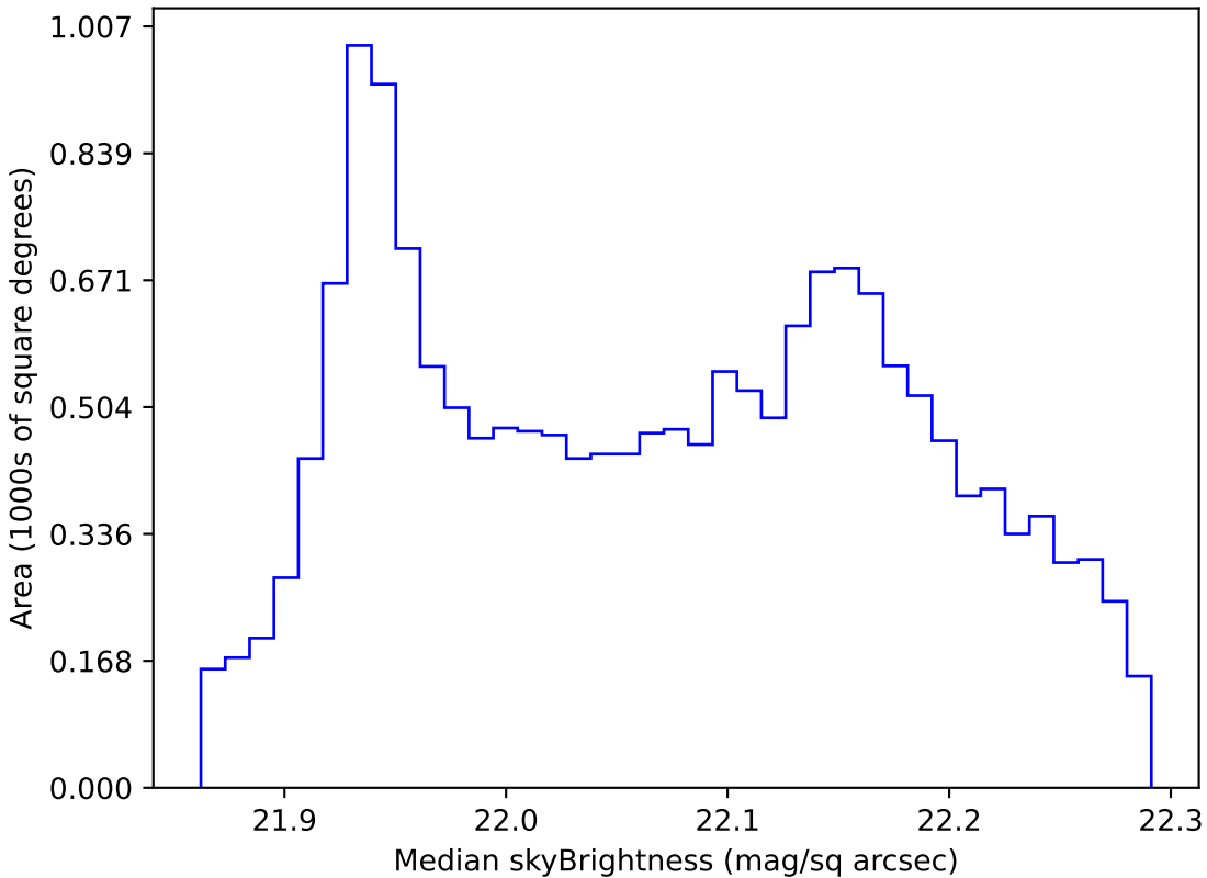
roll_pause_mjdp60_v3.4_10yrs WFD g band: Median skyBrightness
