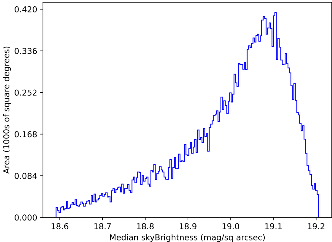
roll_pause_mjdp60_v3.4_10yrs All sky z band: Median skyBrightness
