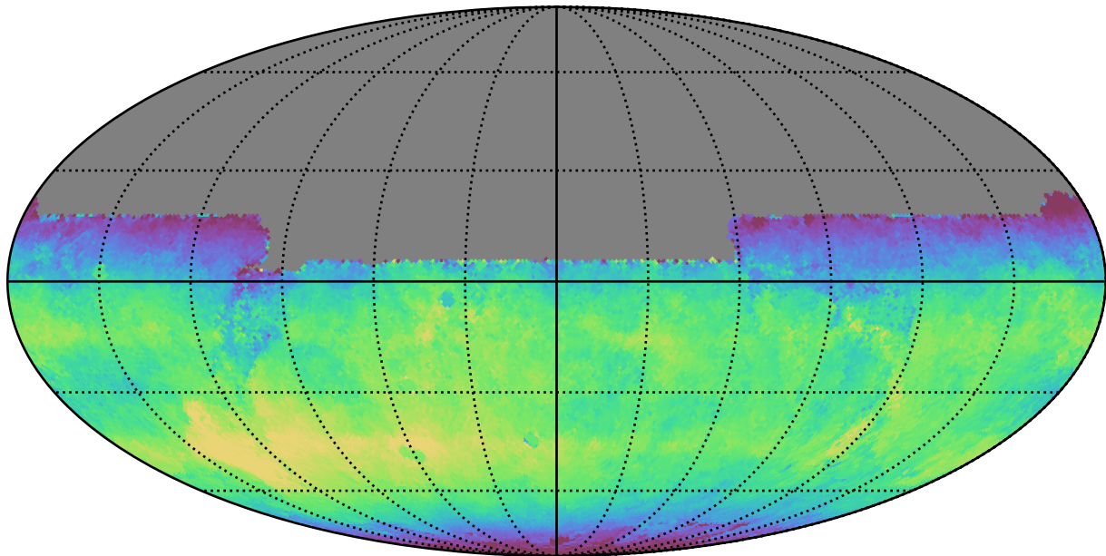
roll_pause_mjdp60_v3.4_10yrs All sky y band: Median skyBrightness
