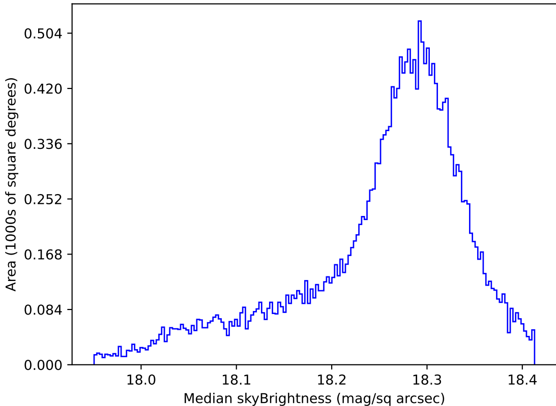
roll_pause_mjdp60_v3.4_10yrs All sky y band: Median skyBrightness
