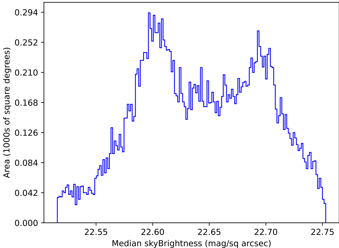
roll_pause_mjdp60_v3.4_10yrs All sky u band: Median skyBrightness
