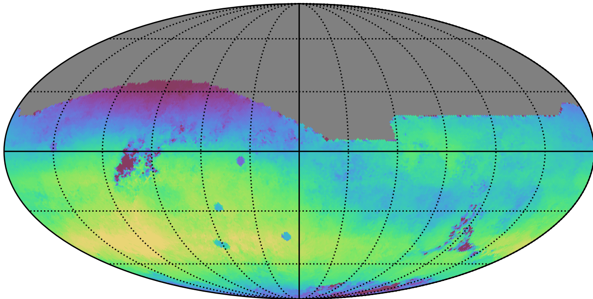
roll_pause_mjdp60_v3.4_10yrs All sky r band: Median skyBrightness
