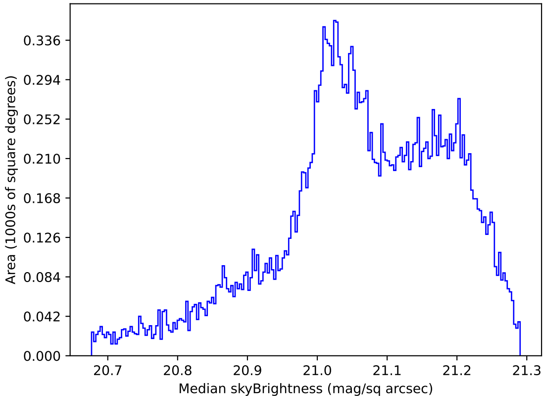
roll_pause_mjdp60_v3.4_10yrs All sky r band: Median skyBrightness
