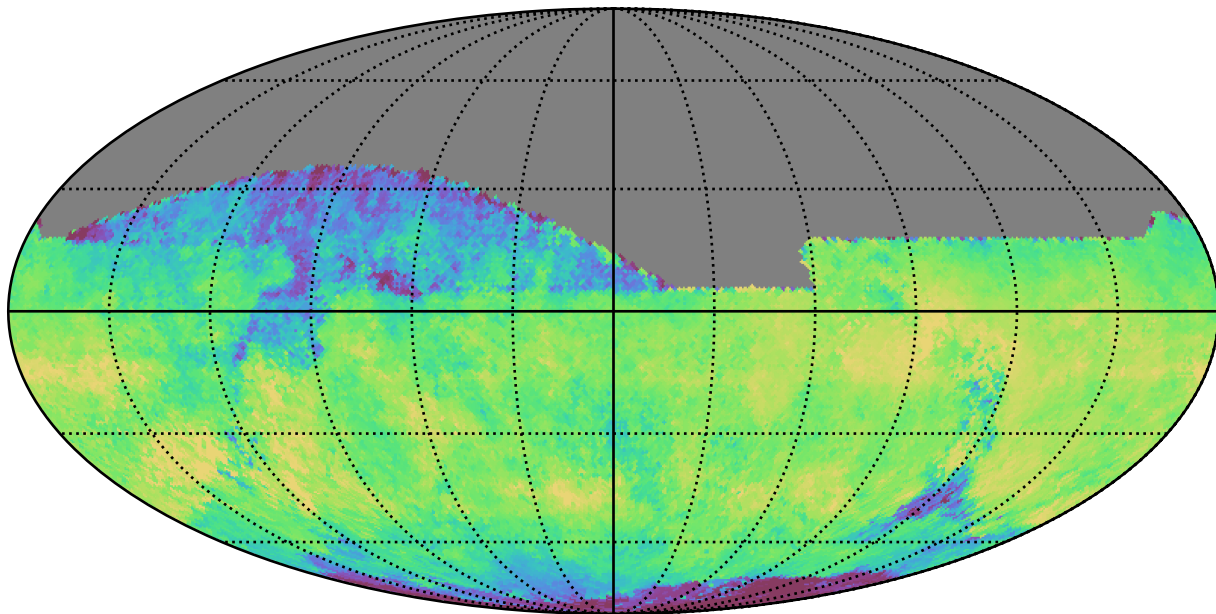
roll_pause_mjdp60_v3.4_10yrs All sky i band: Median skyBrightness
