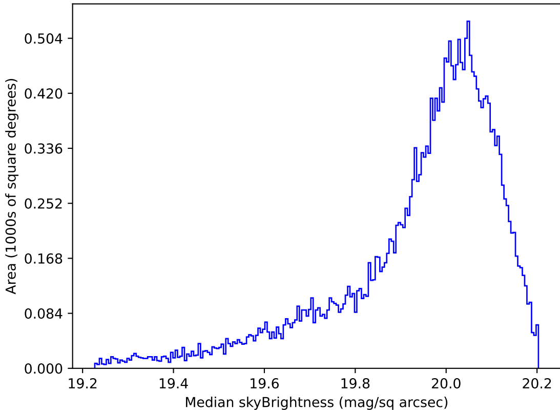
roll_pause_mjdp60_v3.4_10yrs All sky i band: Median skyBrightness
