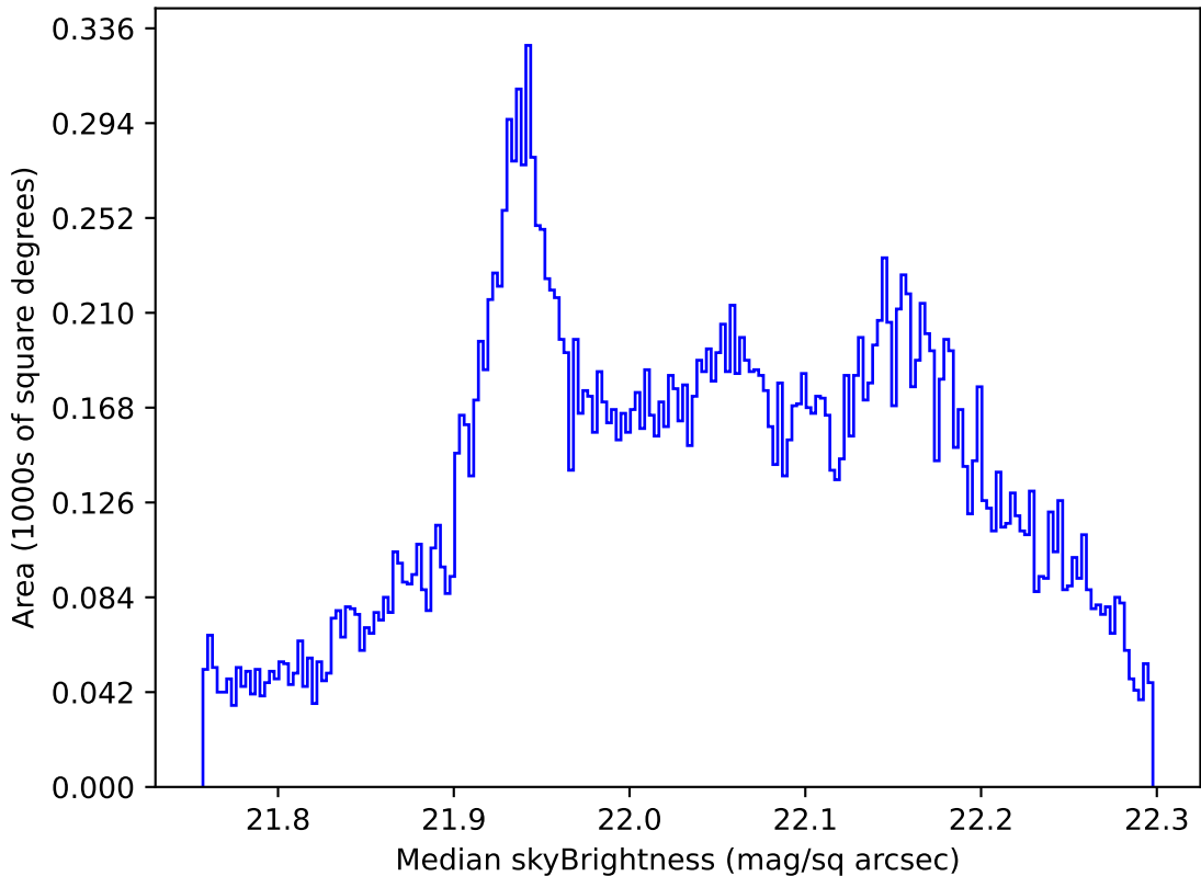
roll_pause_mjdp60_v3.4_10yrs All sky g band: Median skyBrightness
