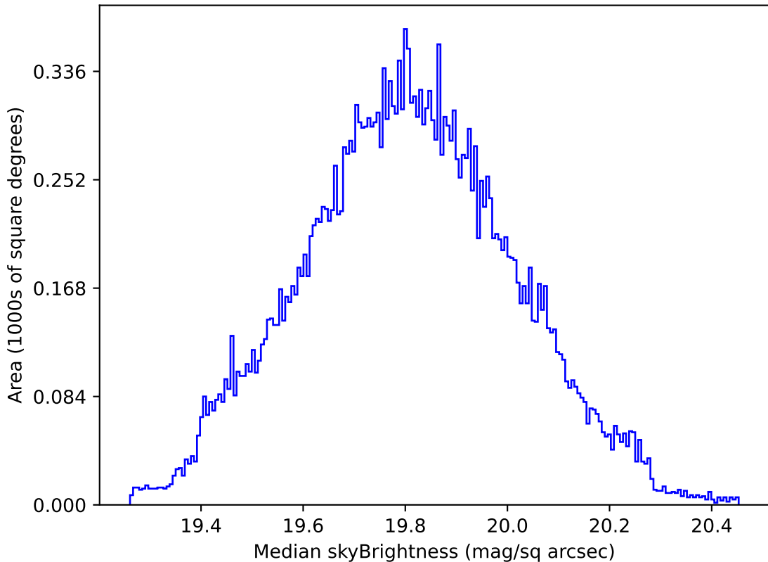
roll_pause_mjdp60_v3.4_10yrs All sky all bands: Median skyBrightness
