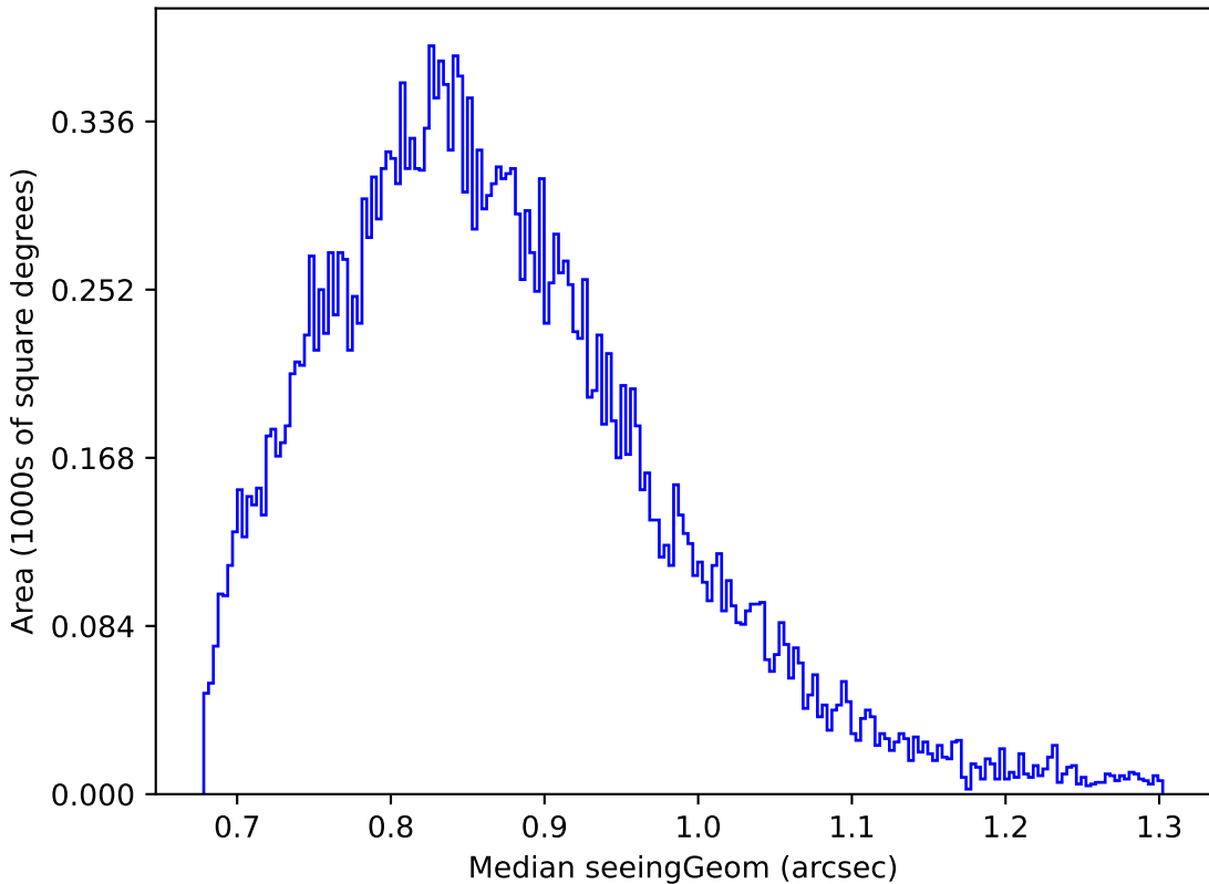
roll_pause_mjdp60_v3.4_10yrs Yr 1 z band: Median seeingGeom
