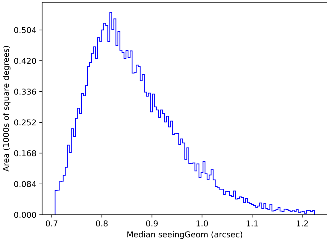
roll_pause_mjdp60_v3.4_10yrs Yr 1 y band: Median seeingGeom
