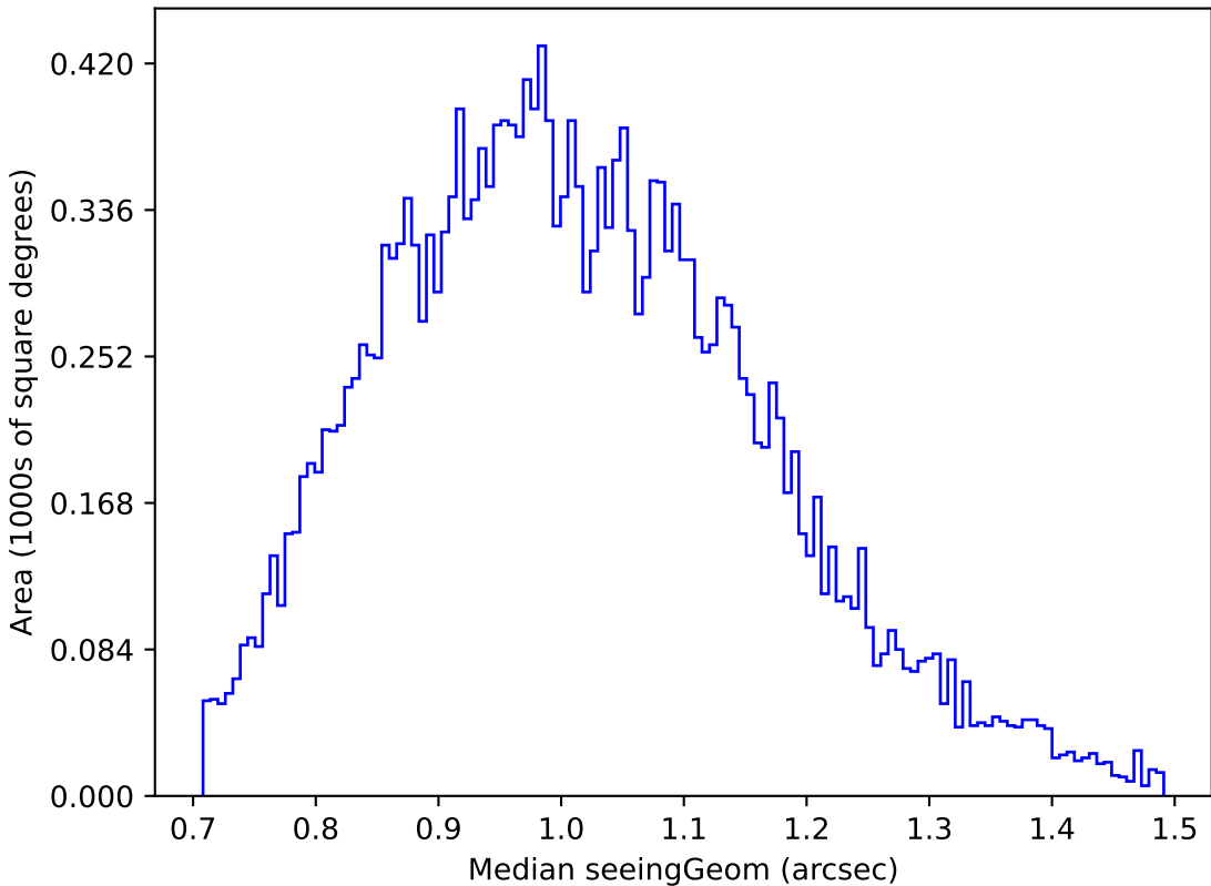
roll_pause_mjdp60_v3.4_10yrs Yr 1 u band: Median seeingGeom
