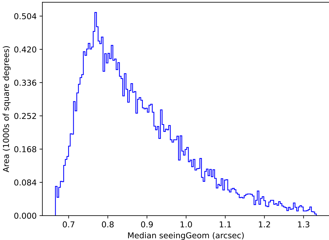
roll_pause_mjdp60_v3.4_10yrs Yr 1 r band: Median seeingGeom
