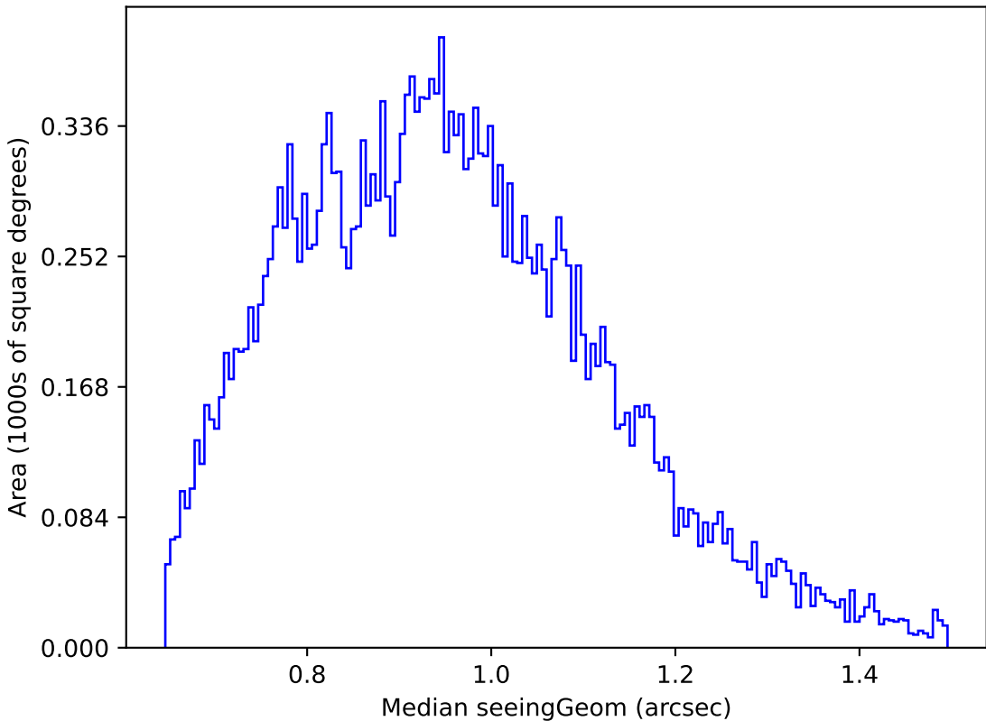
roll_pause_mjdp60_v3.4_10yrs Yr 1 g band: Median seeingGeom
