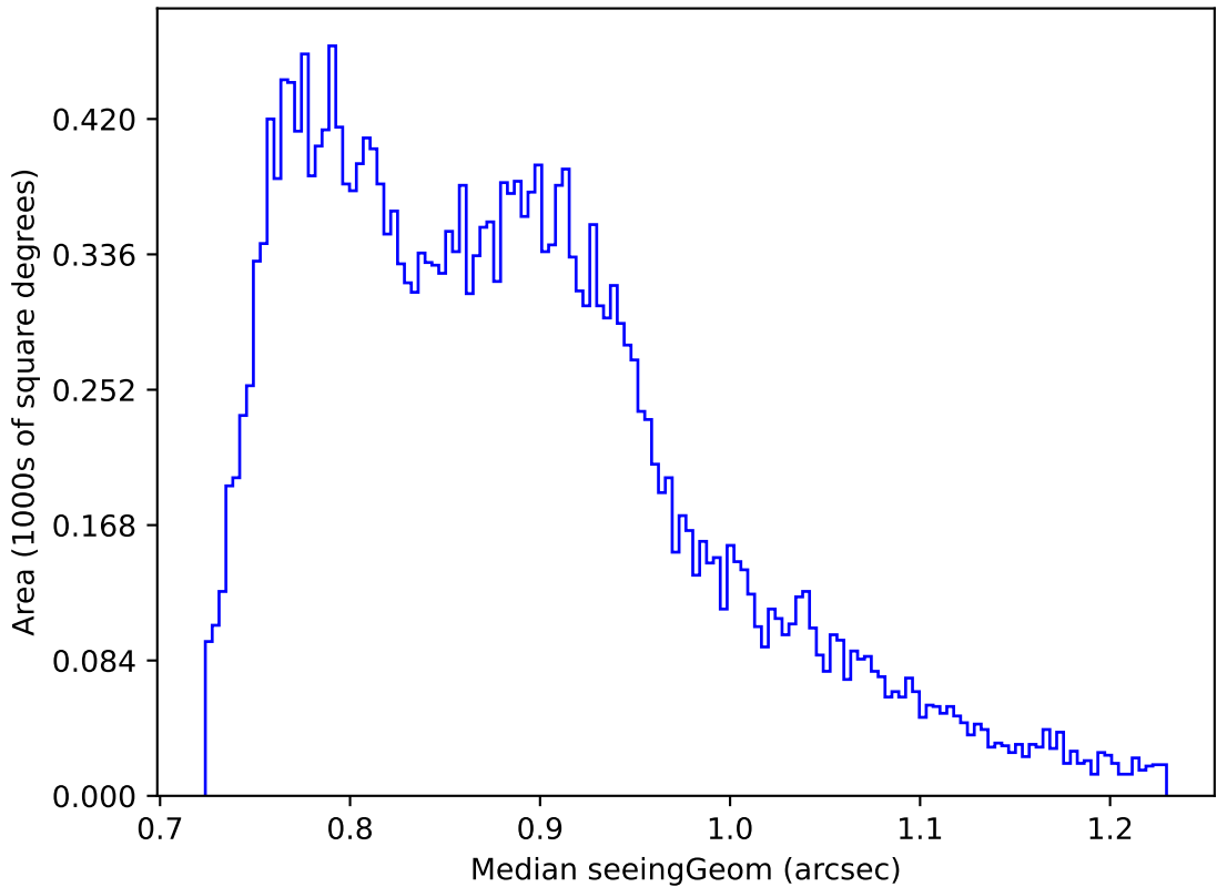
roll_pause_mjdp60_v3.4_10yrs Yr 1 all bands: Median seeingGeom
