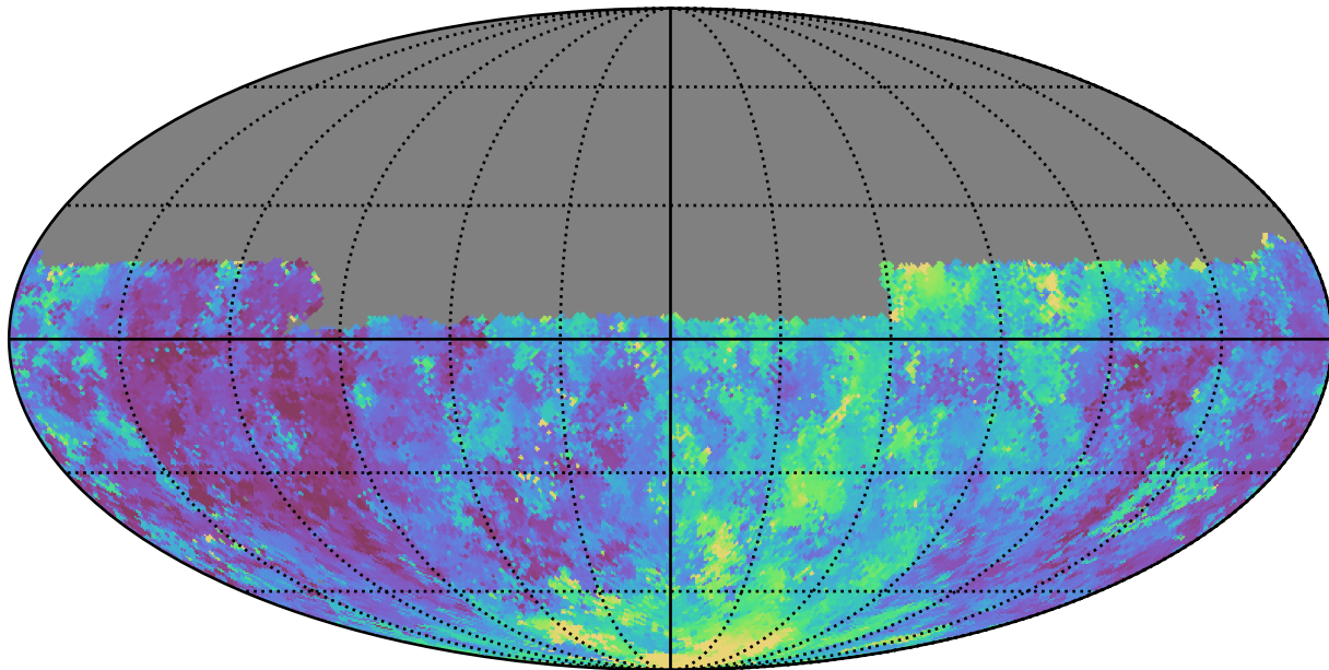
roll_pause_mjdp60_v3.4_10yrs Yr 1 u band: Median seeingEff
