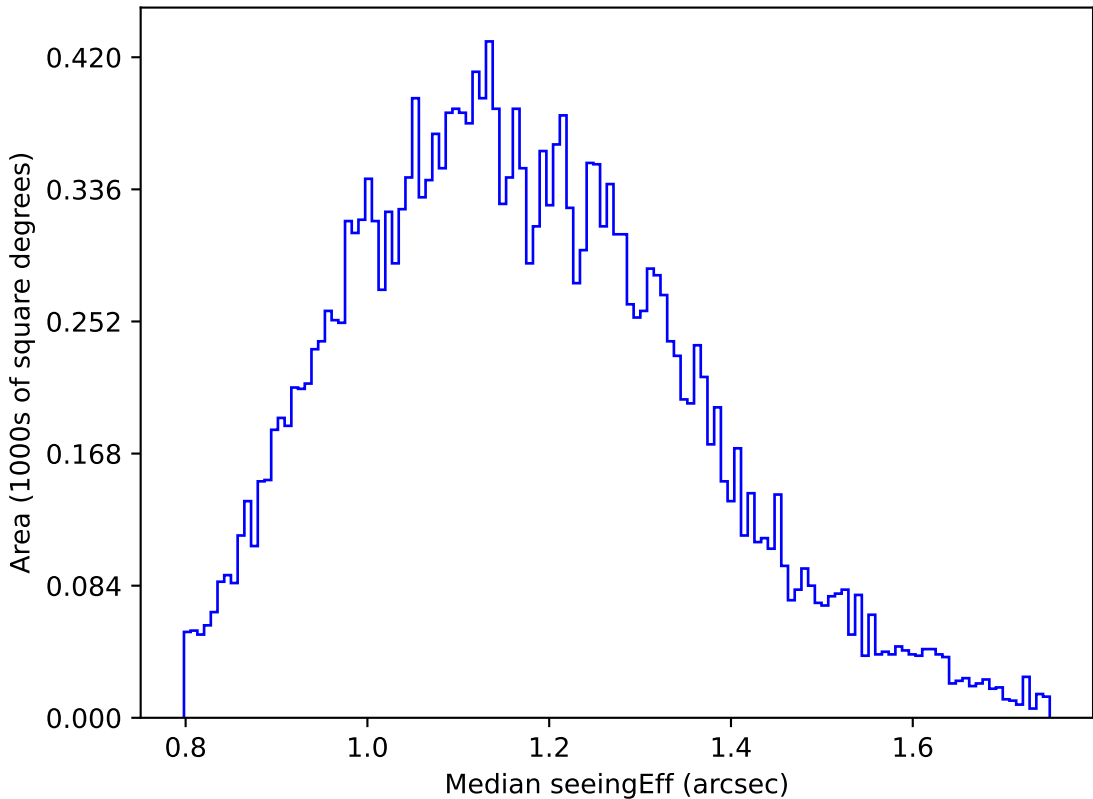
roll_pause_mjdp60_v3.4_10yrs Yr 1 u band: Median seeingEff
