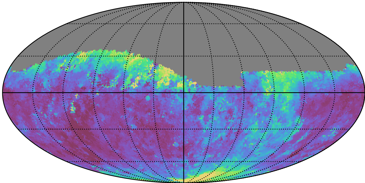
roll_pause_mjdp60_v3.4_10yrs Yr 1 r band: Median seeingEff
