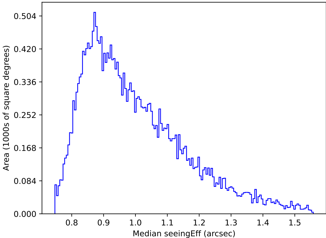
roll_pause_mjdp60_v3.4_10yrs Yr 1 r band: Median seeingEff
