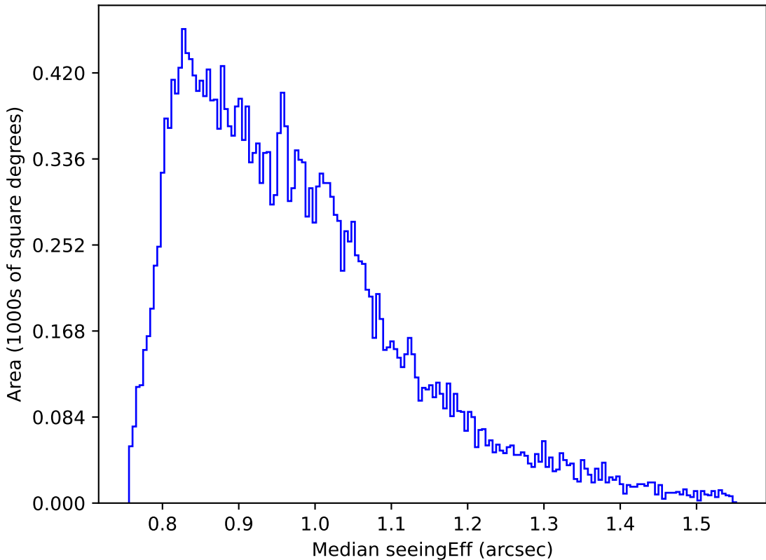
roll_pause_mjdp60_v3.4_10yrs Yr 1 i band: Median seeingEff
