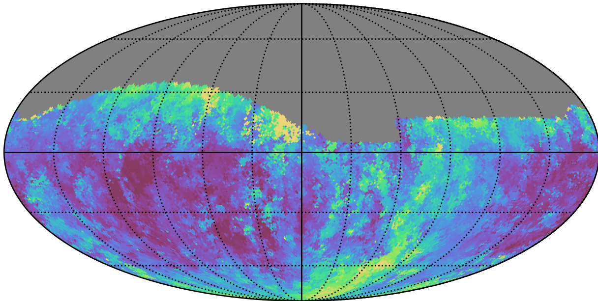
roll_pause_mjdp60_v3.4_10yrs Yr 1 g band: Median seeingEff
