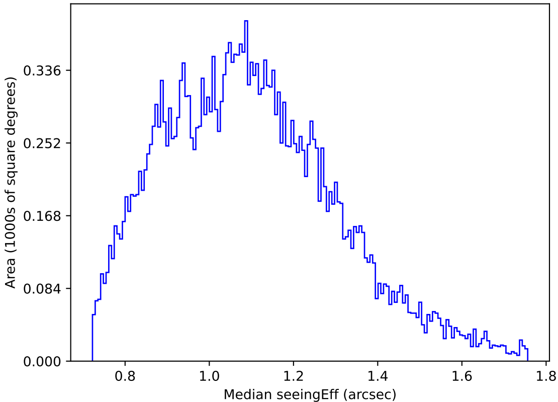
roll_pause_mjdp60_v3.4_10yrs Yr 1 g band: Median seeingEff
