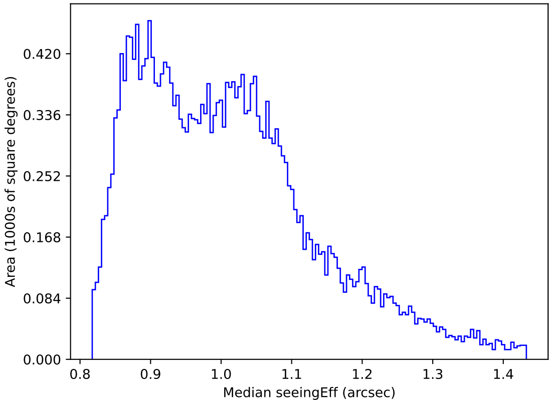
roll_pause_mjdp60_v3.4_10yrs Yr 1 all bands: Median seeingEff
