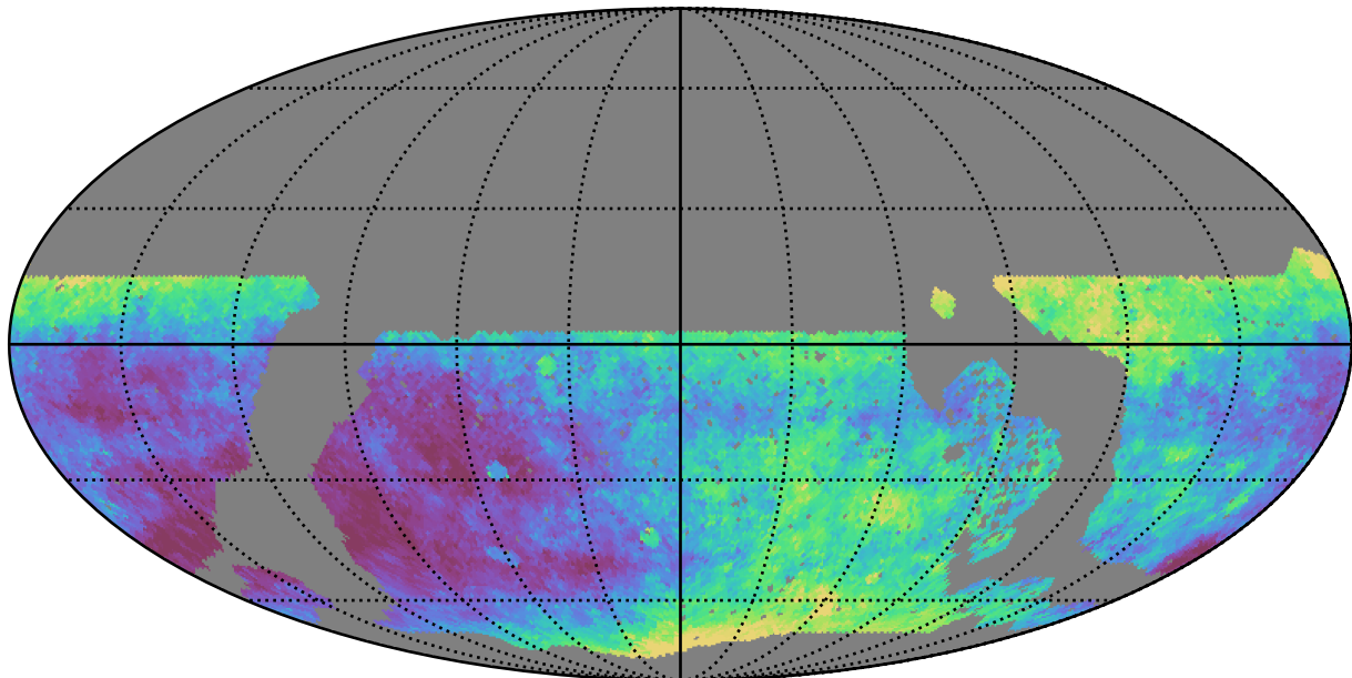
roll_pause_mjdp60_v3.4_10yrs WFD z band: Median seeingEff
