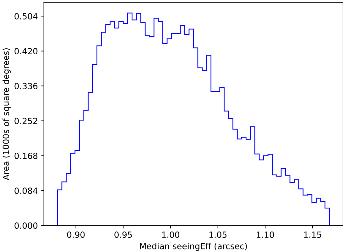
roll_pause_mjdp60_v3.4_10yrs WFD y band: Median seeingEff
