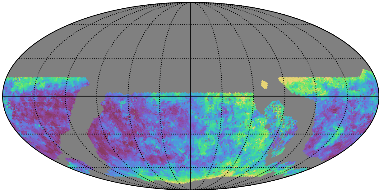
roll_pause_mjdp60_v3.4_10yrs WFD u band: Median seeingEff
