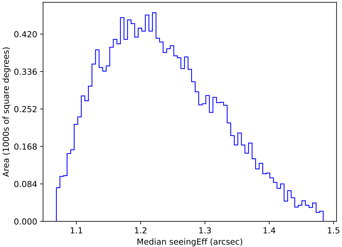
roll_pause_mjdp60_v3.4_10yrs WFD u band: Median seeingEff
