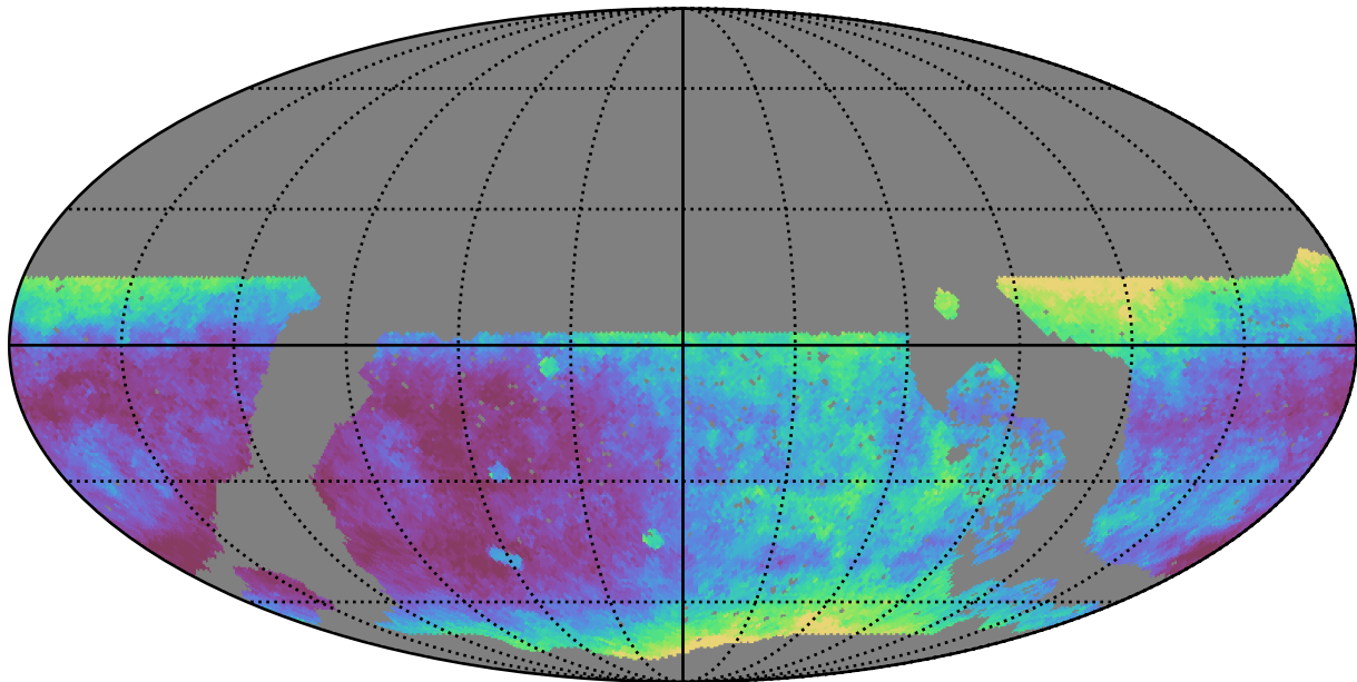
roll_pause_mjdp60_v3.4_10yrs WFD r band: Median seeingEff
