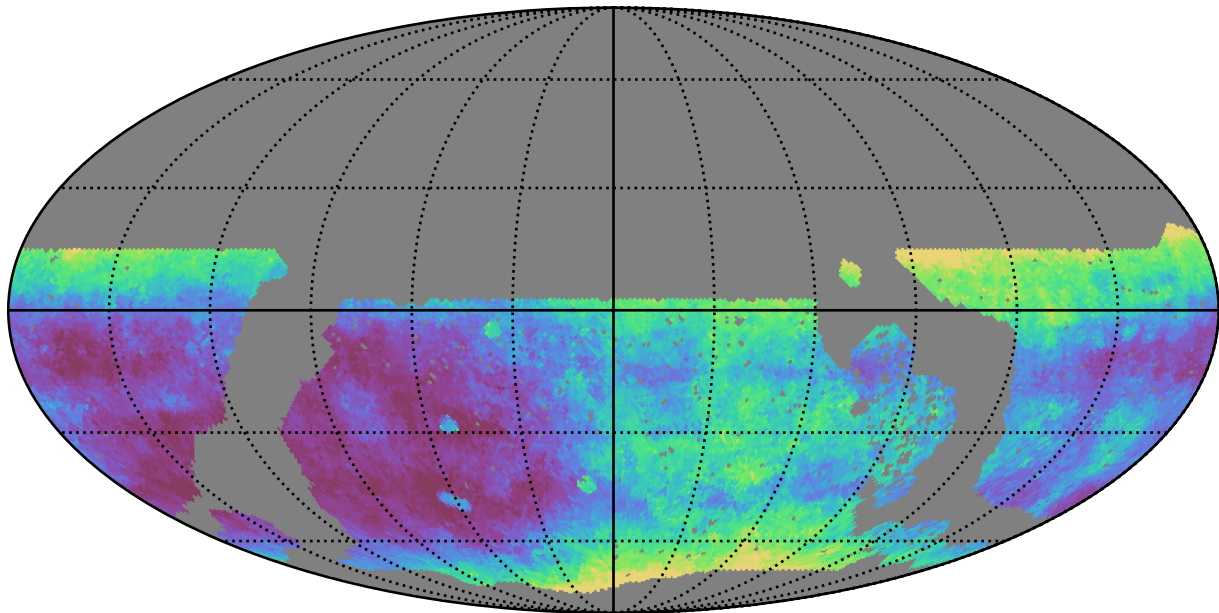
roll_pause_mjdp60_v3.4_10yrs WFD i band: Median seeingEff
