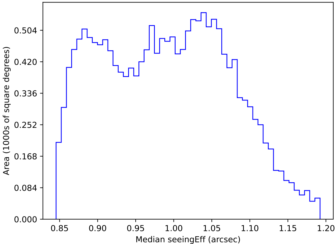
roll_pause_mjdp60_v3.4_10yrs WFD i band: Median seeingEff
