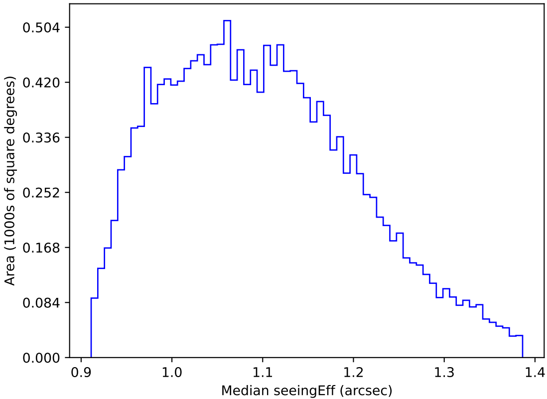
roll_pause_mjdp60_v3.4_10yrs WFD g band: Median seeingEff
