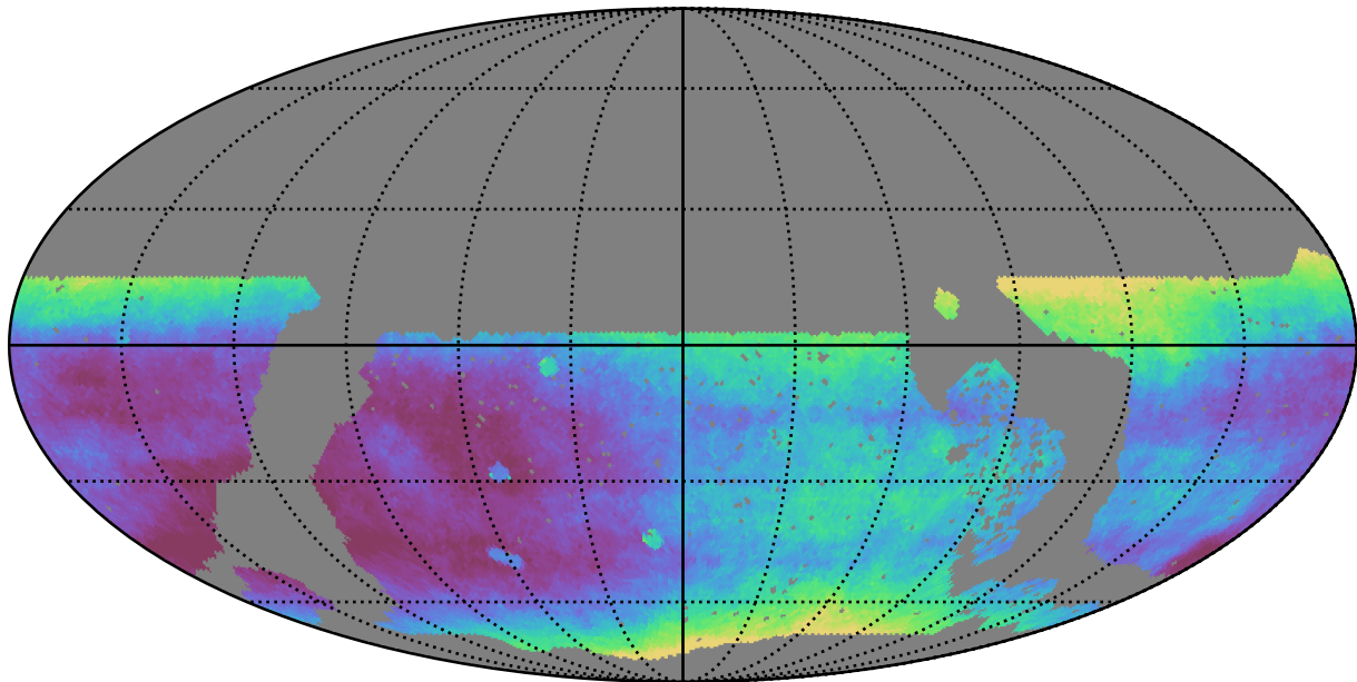
roll_pause_mjdp60_v3.4_10yrs WFD all bands: Median seeingEff
