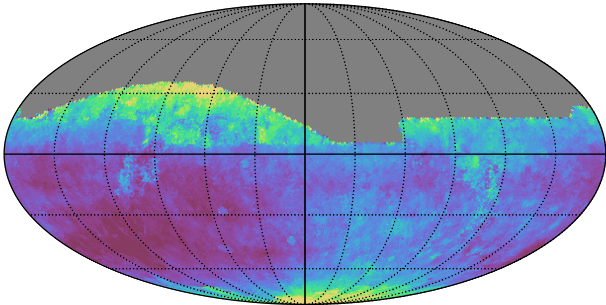
roll_pause_mjdp60_v3.4_10yrs All sky z band: Median seeingEff
