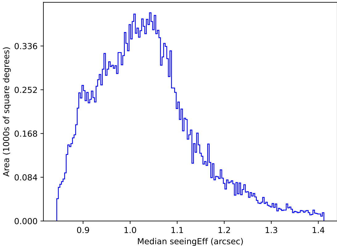
roll_pause_mjdp60_v3.4_10yrs All sky z band: Median seeingEff
