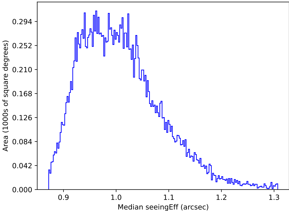
roll_pause_mjdp60_v3.4_10yrs All sky y band: Median seeingEff
