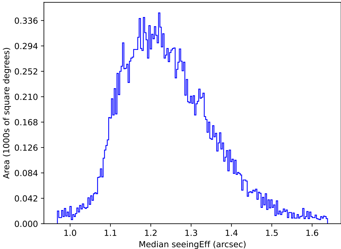
roll_pause_mjdp60_v3.4_10yrs All sky u band: Median seeingEff
