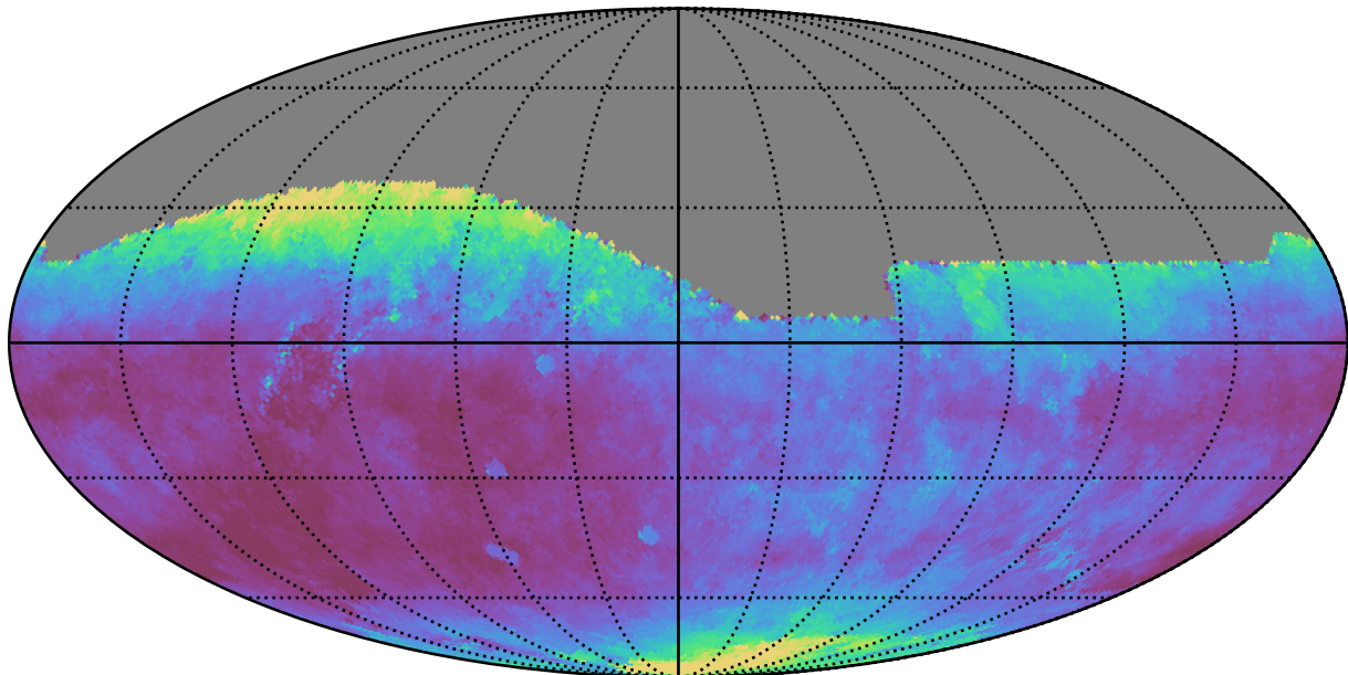
roll_pause_mjdp60_v3.4_10yrs All sky r band: Median seeingEff
