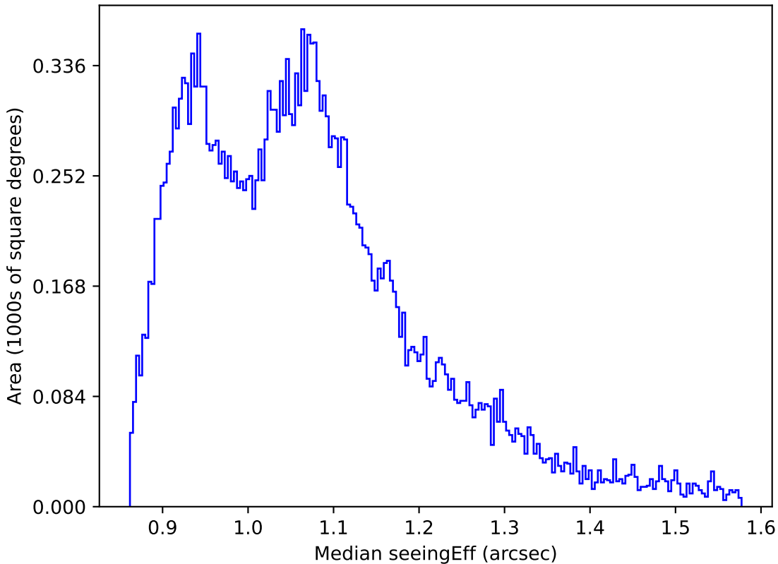
roll_pause_mjdp60_v3.4_10yrs All sky r band: Median seeingEff
