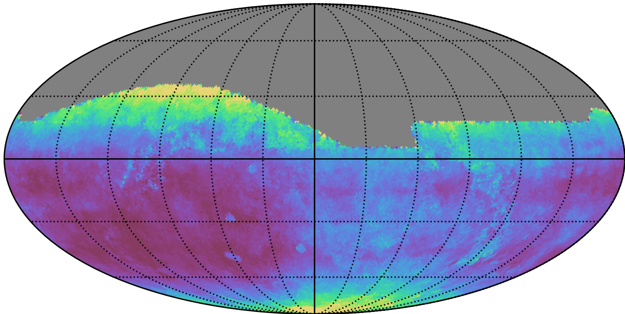
roll_pause_mjdp60_v3.4_10yrs All sky i band: Median seeingEff
