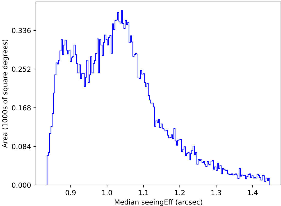
roll_pause_mjdp60_v3.4_10yrs All sky i band: Median seeingEff
