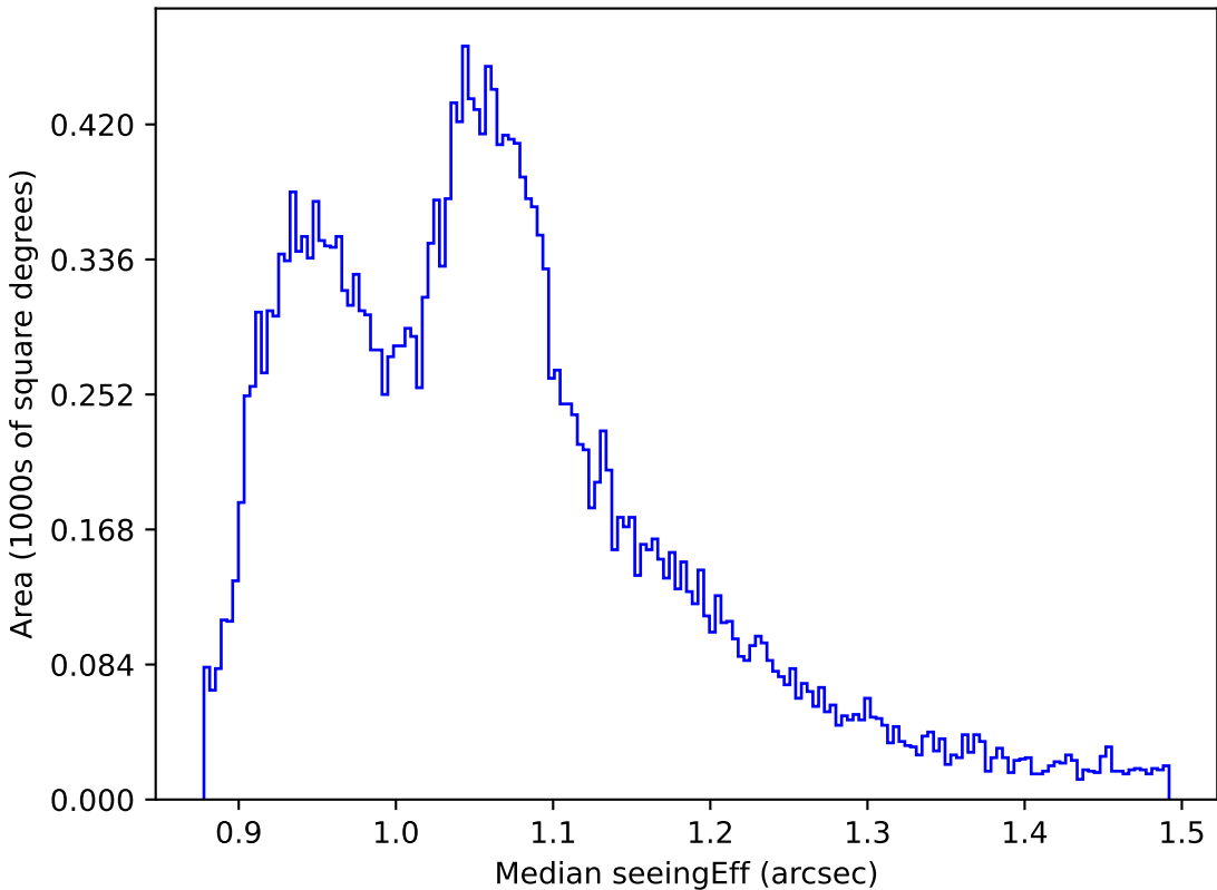
roll_pause_mjdp60_v3.4_10yrs All sky all bands: Median seeingEff
