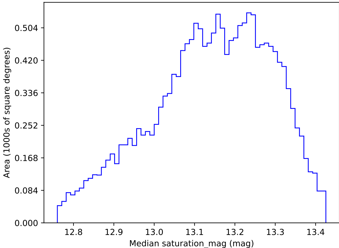
roll_pause_mjdp60_v3.4_10yrs WFD y band: Median saturation_mag
