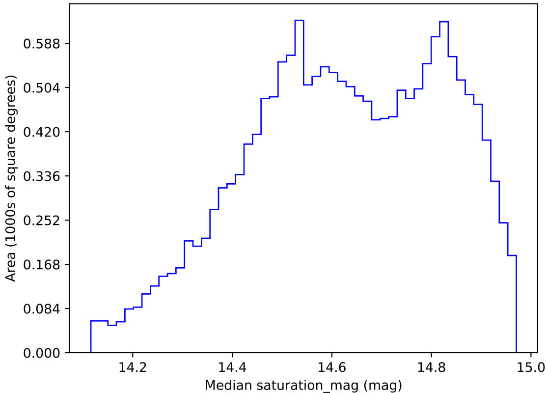
roll_pause_mjdp60_v3.4_10yrs WFD r band: Median saturation_mag
